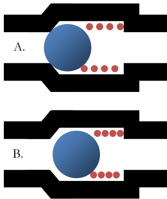
Figure 7: Ball check valve, closed in A, open in B. Image redrawn from Dr. Frank Fronczak, PhD. (2009), personal communication.
