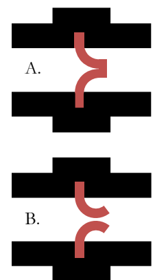
Figure 6: Double flapper valve, closed in A, open in B.
