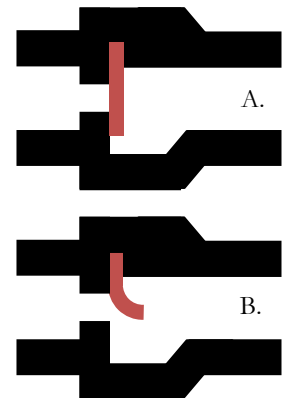
Figure 8: Diaphragm valve, closed in A, open in B.
