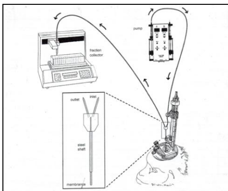
Figure 1: Experimental Setup for Microdialysis
