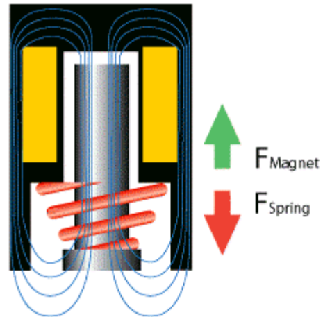
Figure 11. Basic forces in a push/pull solenoid.[19]
