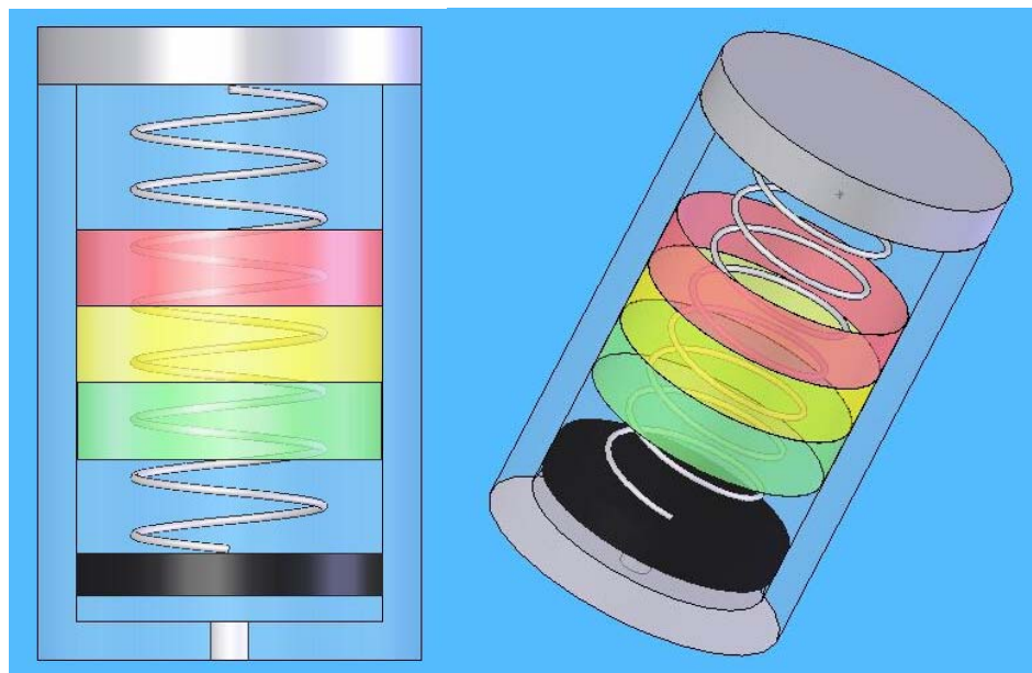
Figure 1.4 Revised Mechanical Spring Schematic
