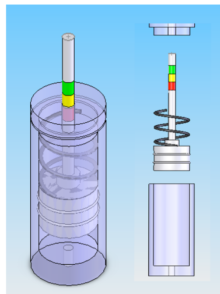
Figure 1.3 Mechanical Spring Design (Endotracheal 17)
