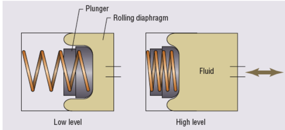
Figure 1.7 Rolling Diaphragm
