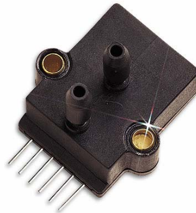
Figure 1.5 Omega PX137-001DV Low Cost Silicon Pressure Sensor with Millivolt Output
