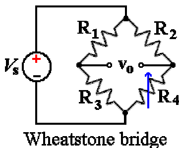
Figure 1.6 Wheatstone Bridge
