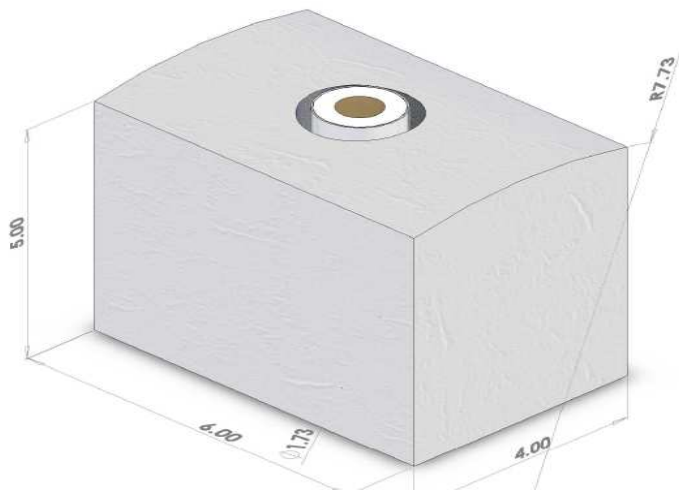
Figure 12: A representative portion of the rubber cast model. The entire model is made of a single soft polymer. All measurements are in inches.
