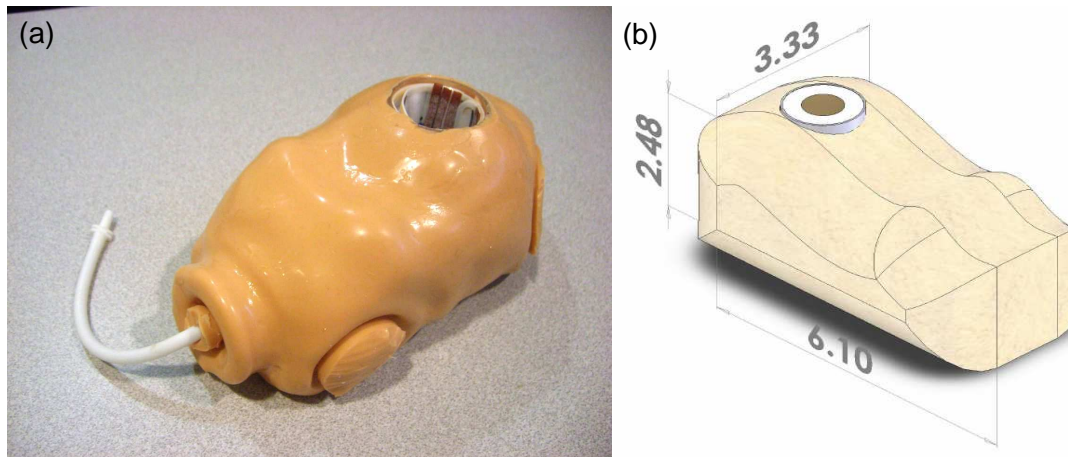
Figure 15: (a) The final prototype. Details of its construction are provided at Appendix B. (b) A technical drawing depicting the dimensions of the prototype. All measurements are in inches.
