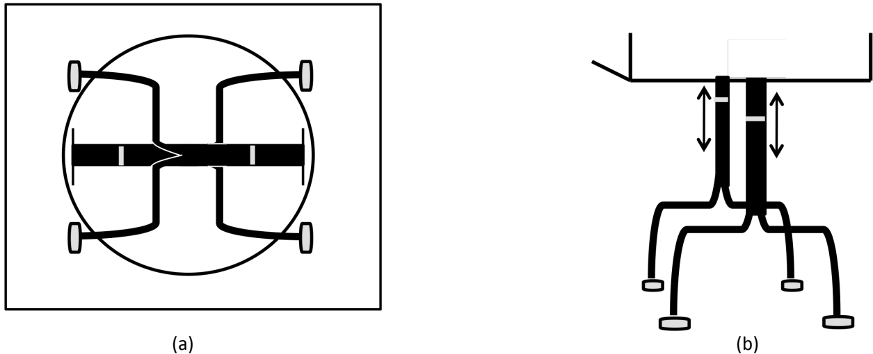
Figure 5: Adjustable legs design: (a) bottom view, (b) side view
