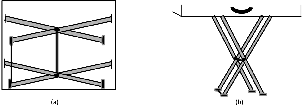
Figure 6: Collapsible legs design: (a) bottom view, (b) side view
