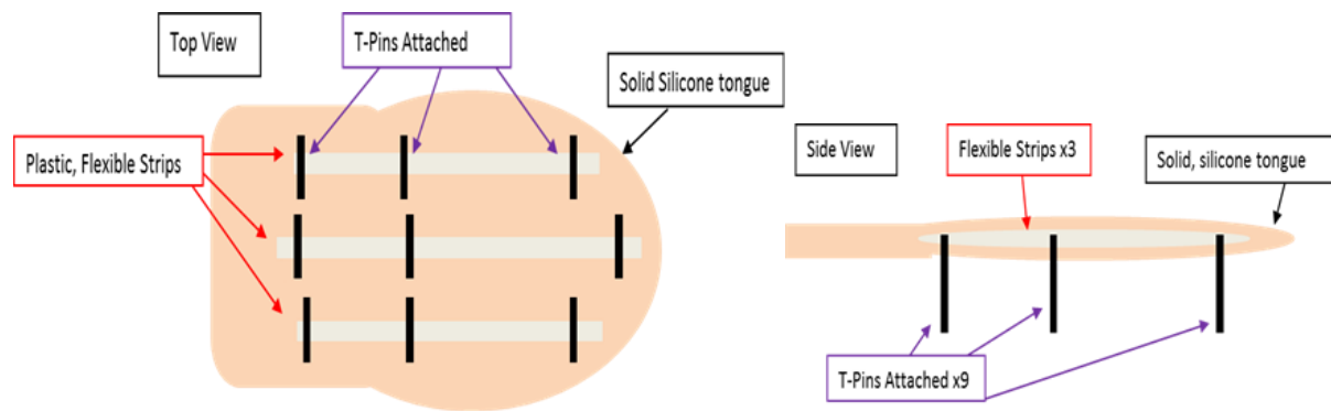
Figure 5: Side and top views of 3-Banded tongue design.
